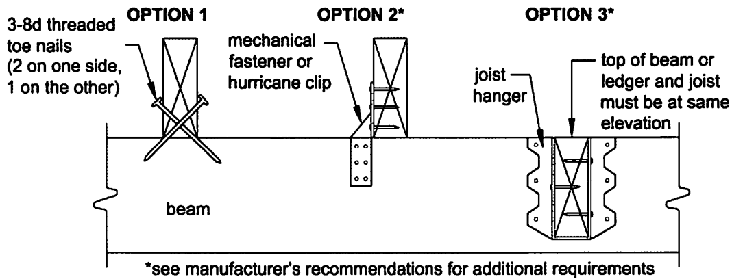
Figure 6. Joist-to-Beam Detail.
