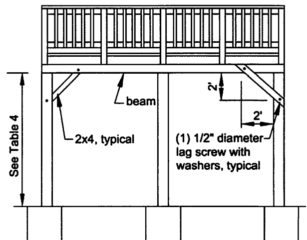
Figure 10. Diagonal Bracing.
