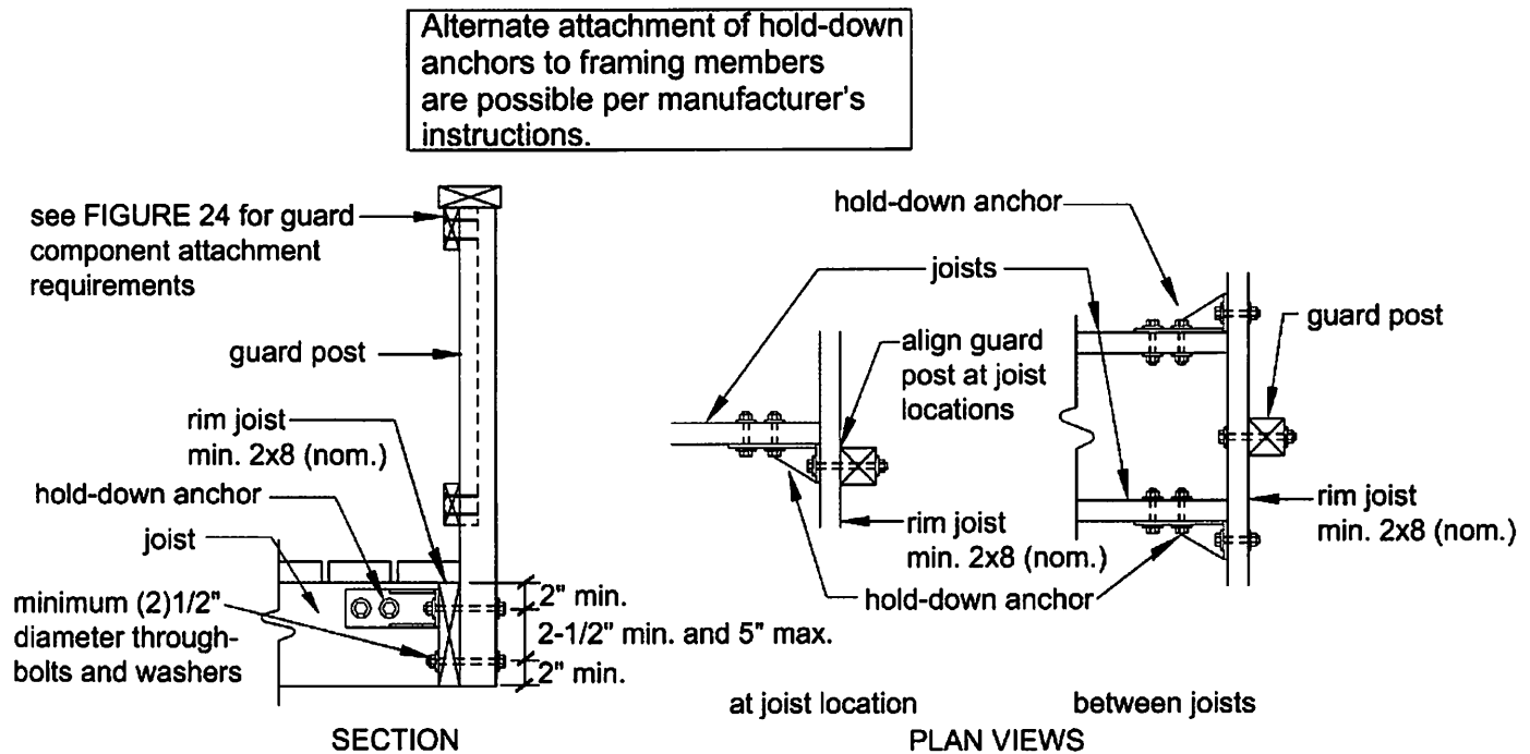
Figure 26. Guard Post to Rim Joist Example.
