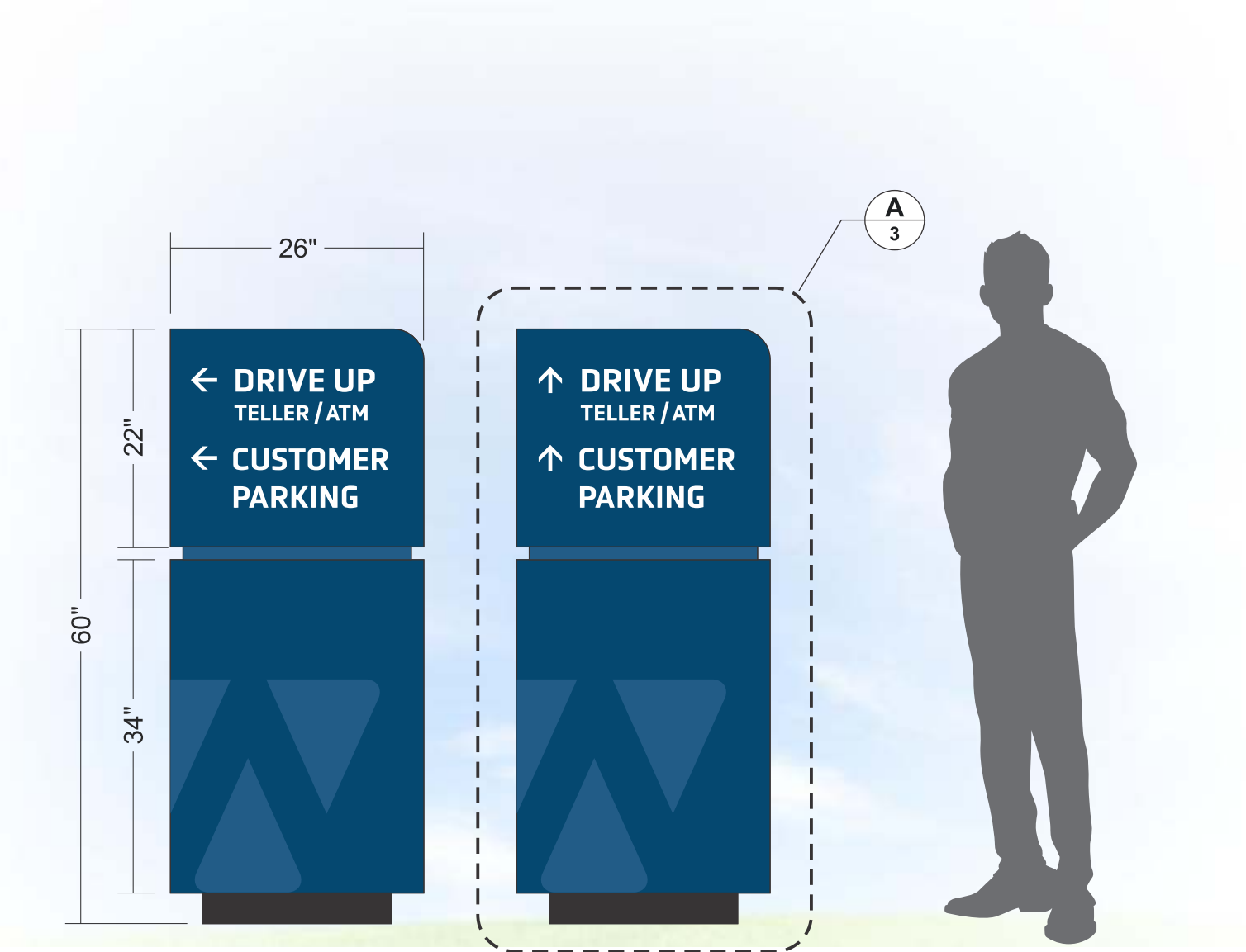
Detail Scale: 3/4"=1'
